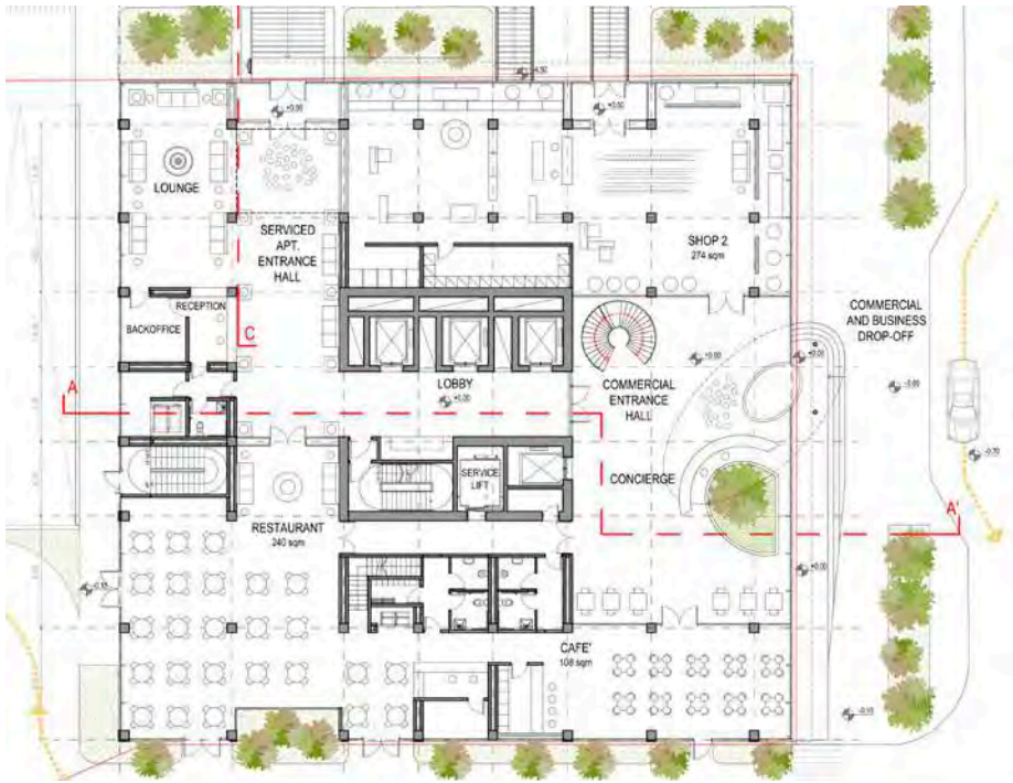
Plan level 2
