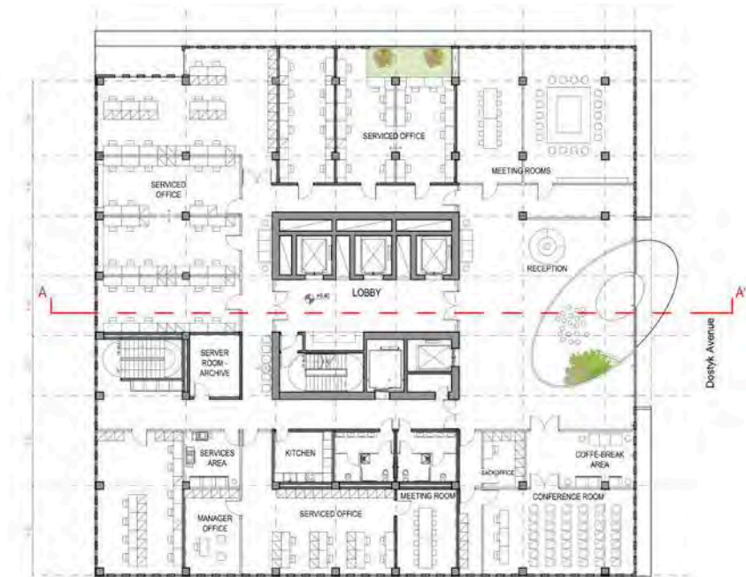
Plan level 3
